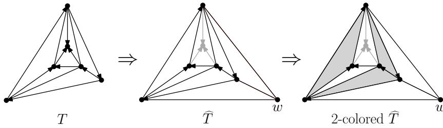
FIGURE 1. The 2-colored auxiliary triangulation \widehat{T} of a triangulation T .
